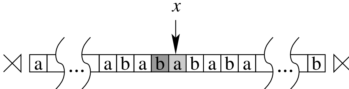
Figure 2: A stringset is Strictly 2-Local if the well-formedness of each word can be determined by checking whether each symbol x in the word is licensed by the preceding symbol.
