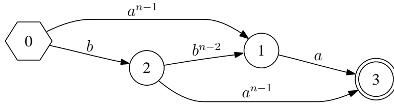
Figure 6.1: A Schema for an Acceptor for L = \{a^n, b^{n-1}a, ba^{n-1}\}
