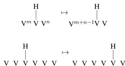
Figure 6: ARs for unbounded shift in Zigula.
